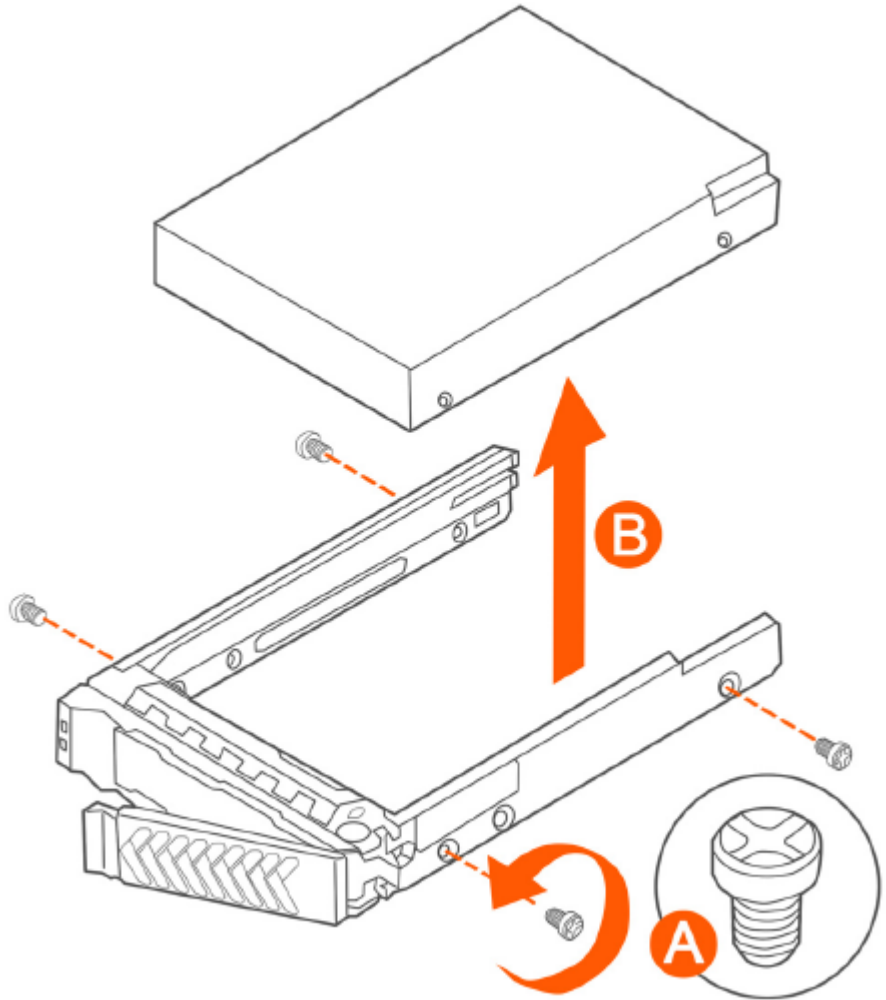
FIGURE 313 Removing the hard drive
