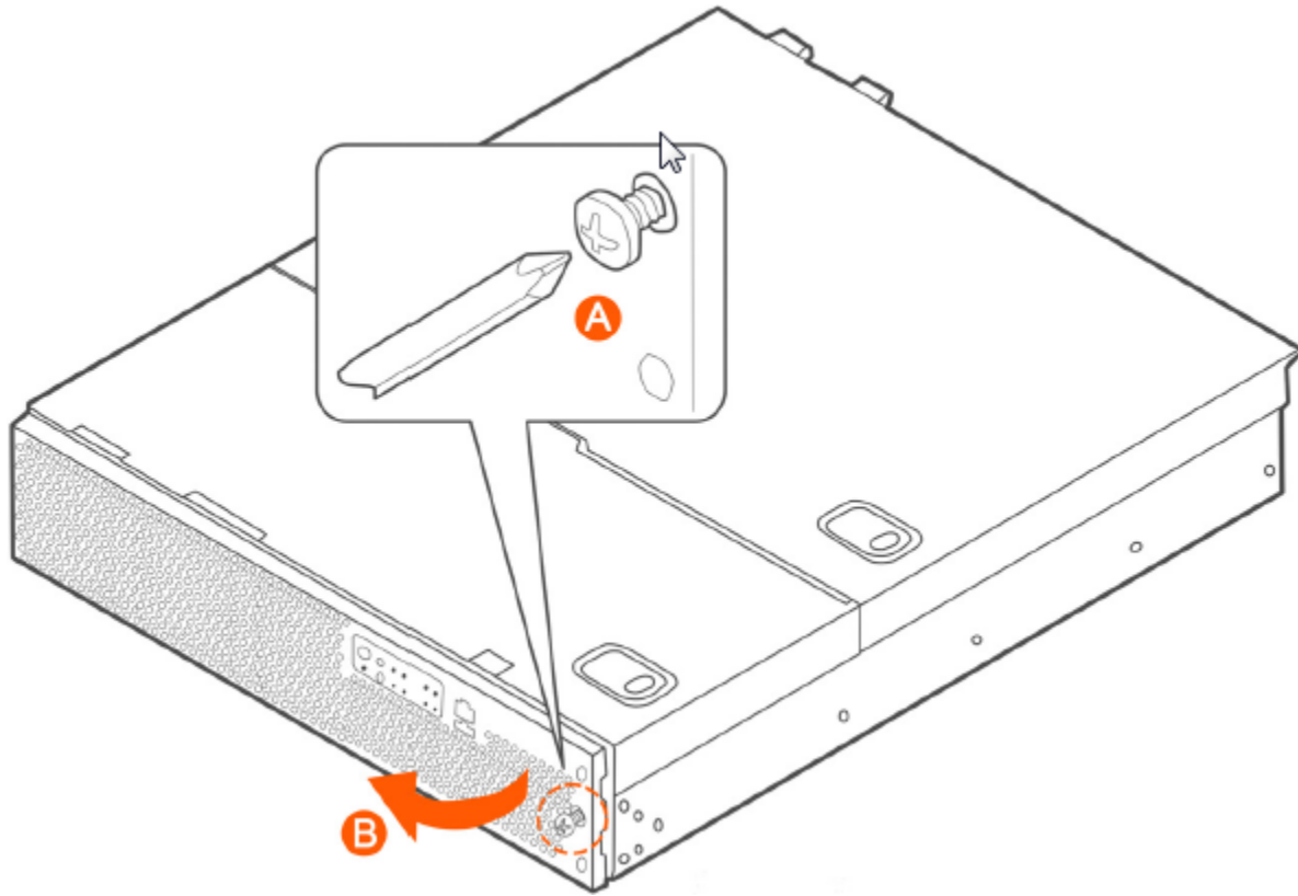
FIGURE 311 Removing the front bezel
