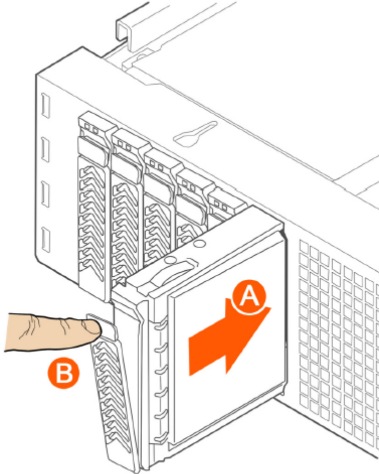
FIGURE 315 Inserting the carrier back into the chassis
