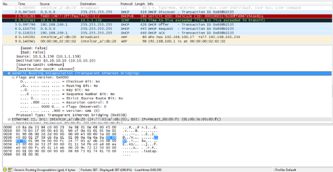
FIGURE 309 Example of SoftGRE packet format
